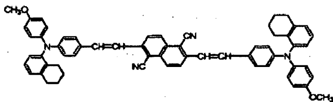
Structural formula (17)-3:
